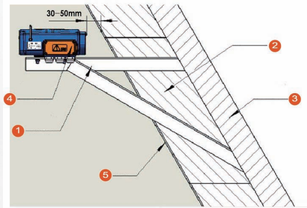
Installation diagram of CAS
