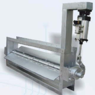
Pneumatic Cylinder Operated Square / Rectangular Damper
