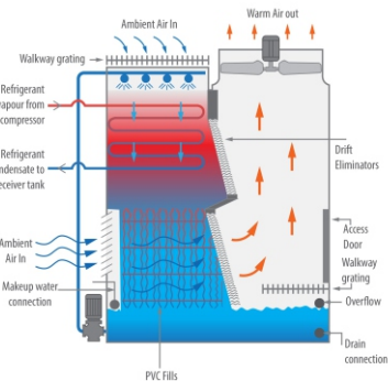
Evaporative Condensers
