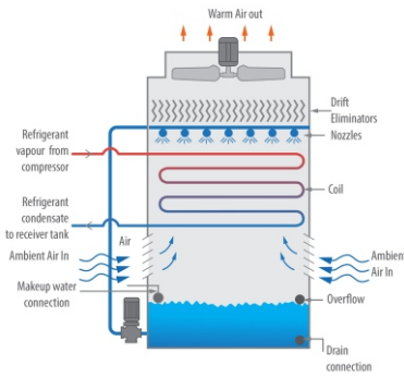
Evaporative Condensers
